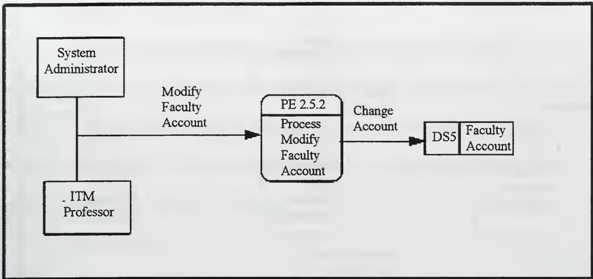
Figure 12. Primitive Level DFD For Maintaing Faculty Account
